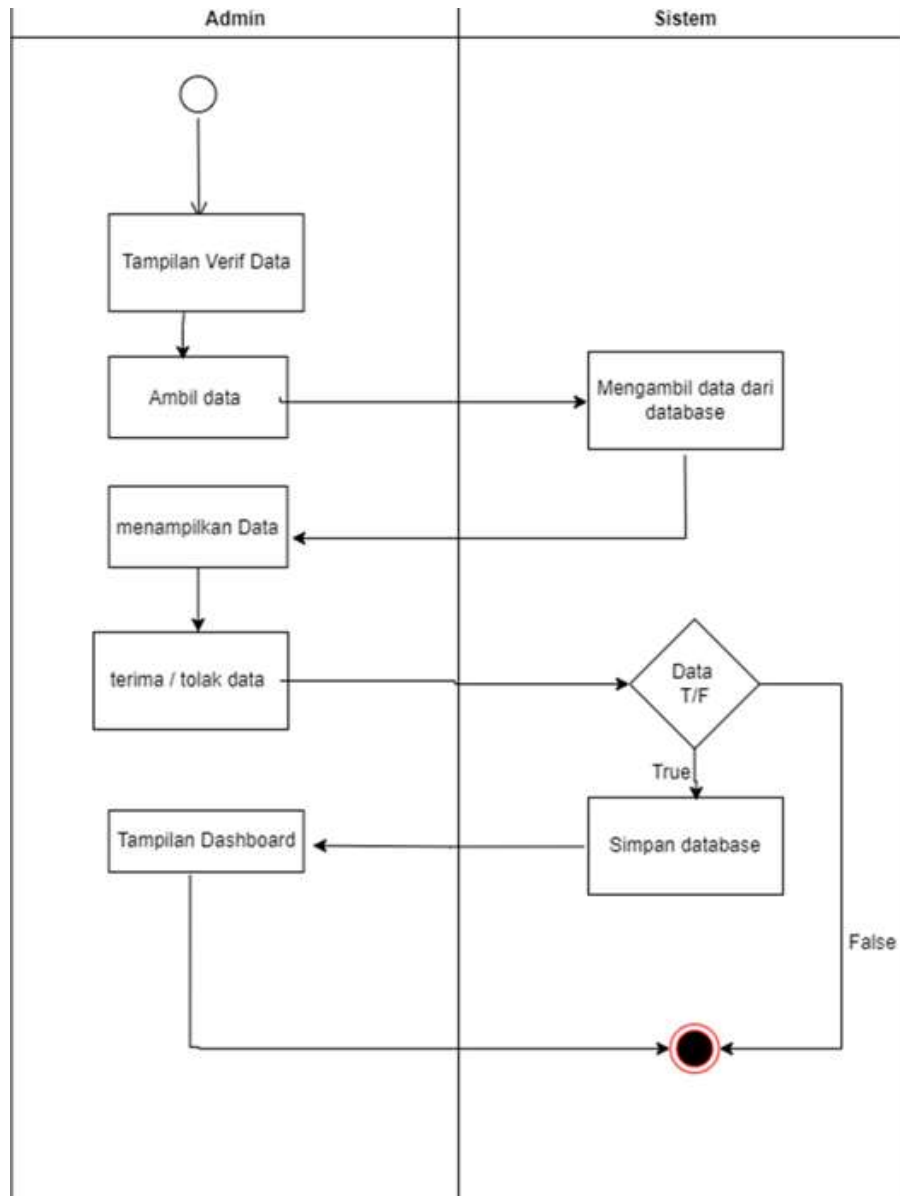
Fig. 4 Activity Diagram Accept or reject data
