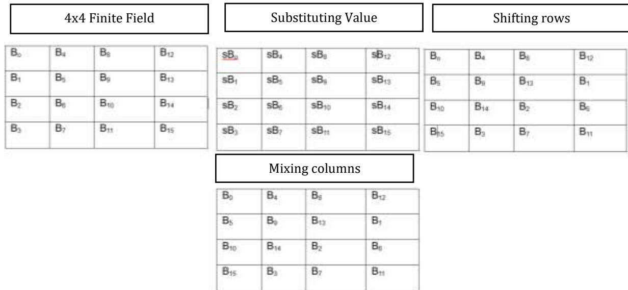
Fig. 6 AES Process Diagram
