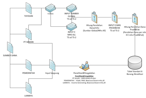
Gambar 1. Workflow Perhitungan Penerimaan Dana
